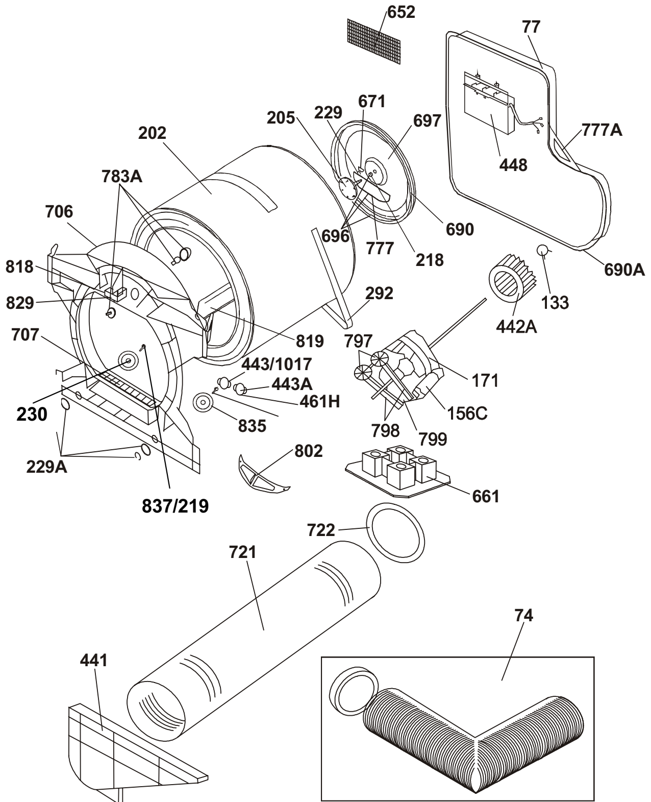
DRUM ASSY - vented
