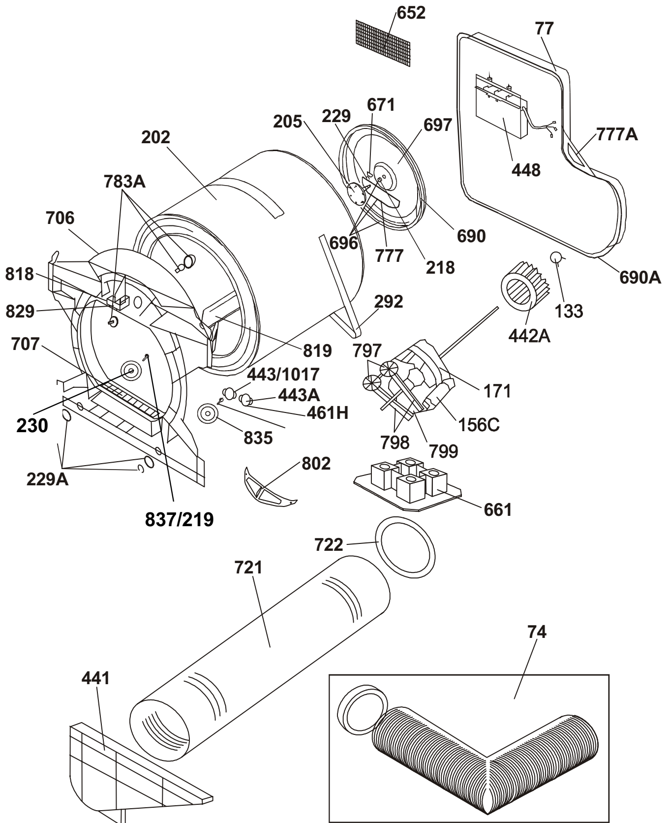
DRUM ASSY - vented
