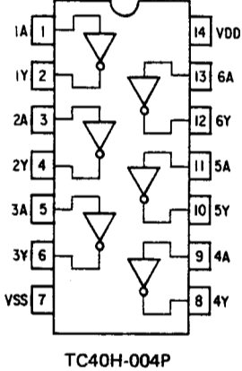
TC40H-004P
