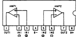
M5218L
