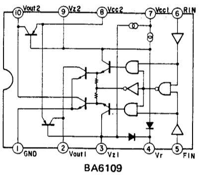
BA6109
