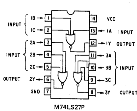
M74LS27P
