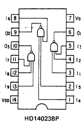
HD14023BP
