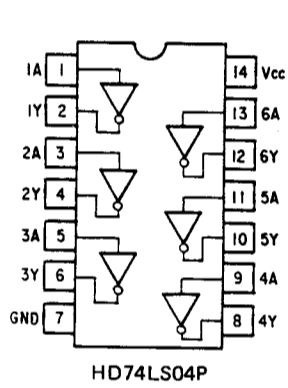
HD74LS04P
