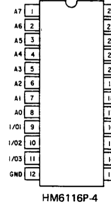
HM6116P-4
