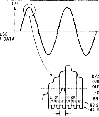
FIG. 8 D/A OUTPUT WAVEFORM
