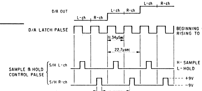
FIG. 7 TIMING CHART OF D/A OUTPUT AND SAMPLE HOLD
