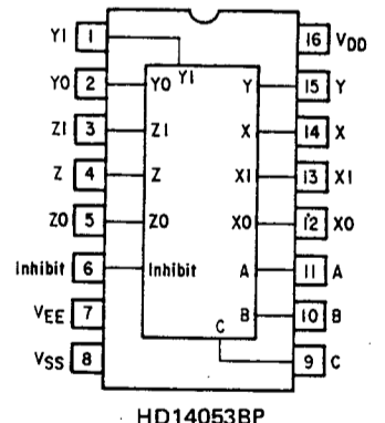
HD14053BP
