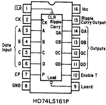
HD74LS161P
