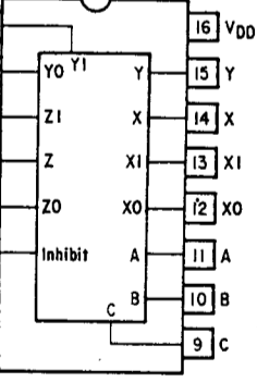
HD14053BP
