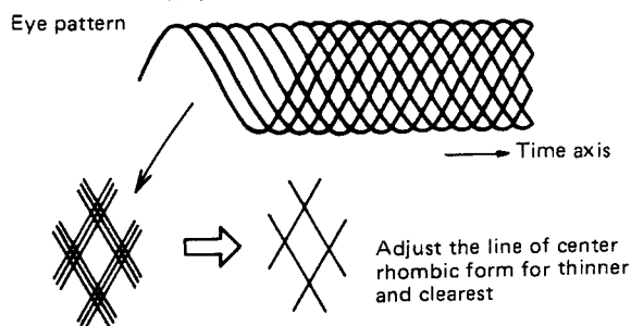
EYE PATTERN FOR (11)
