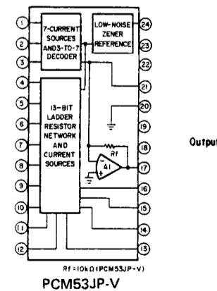
PCM53JP-V
