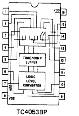
TC4053BP
