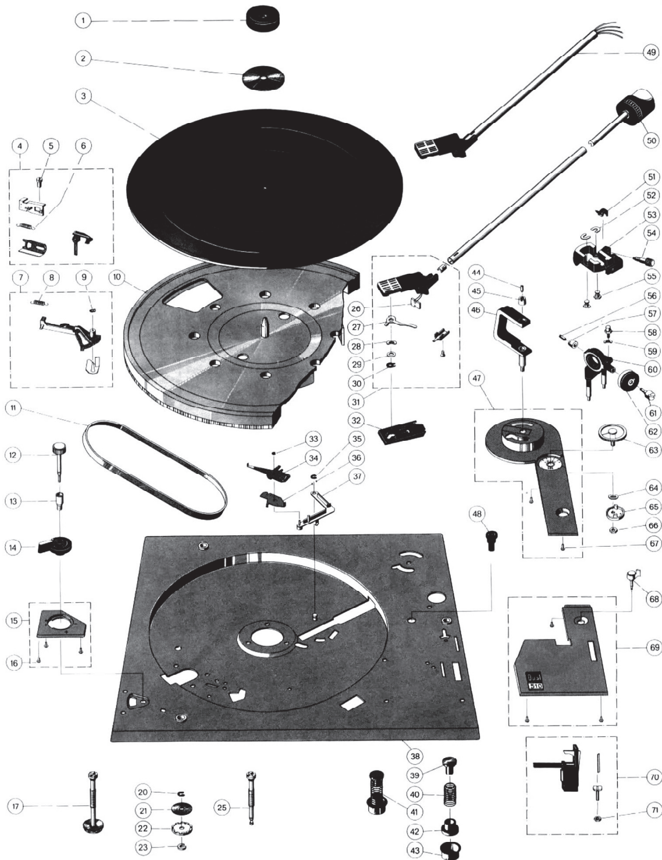
Fig. 19 Exploded view above chassis
