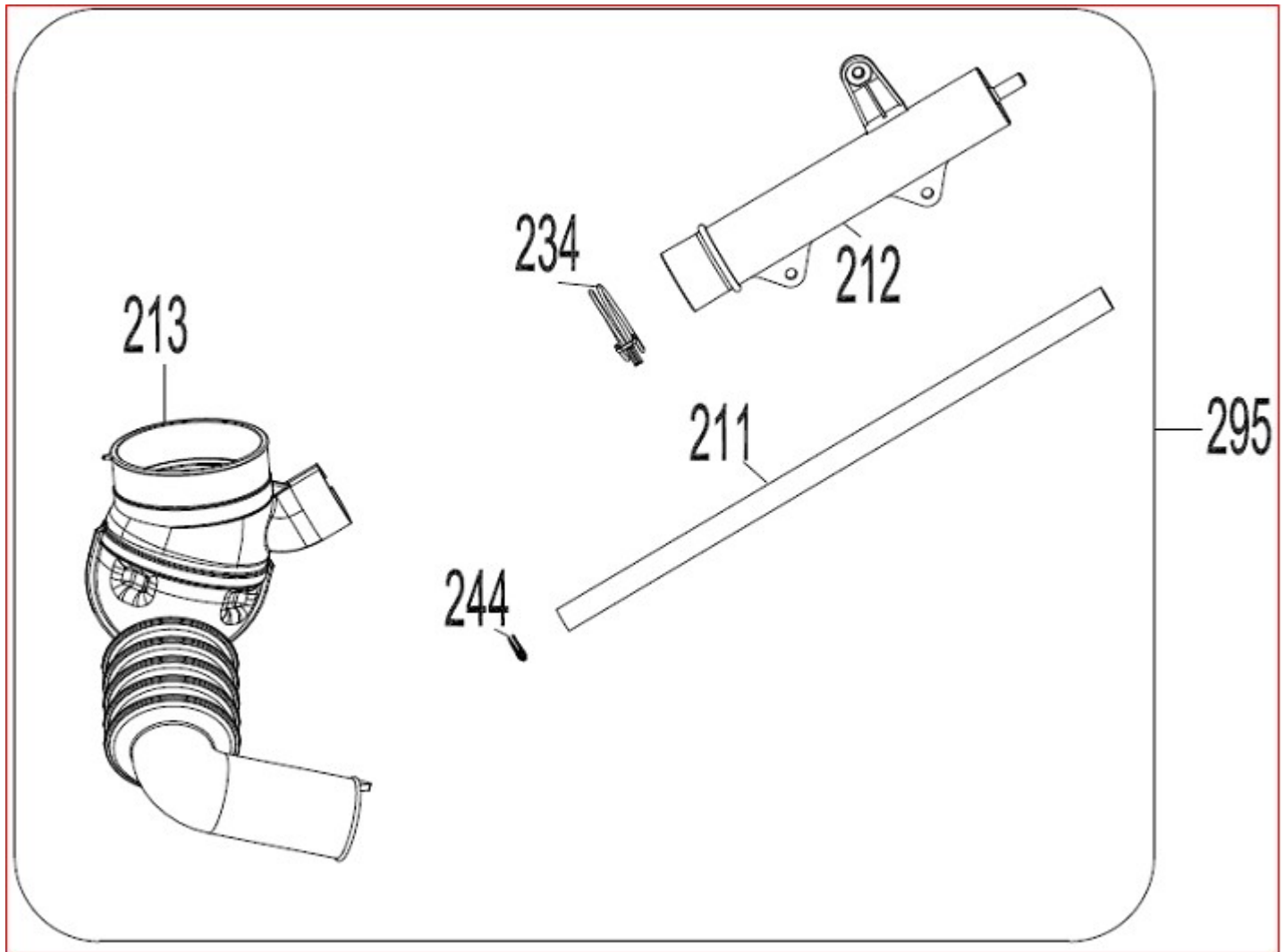
213-212-211-234-244----- PRESSURE SWITCH HOSE GROUP
