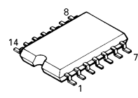
TC74HCT7007AF TC74HC02AF
