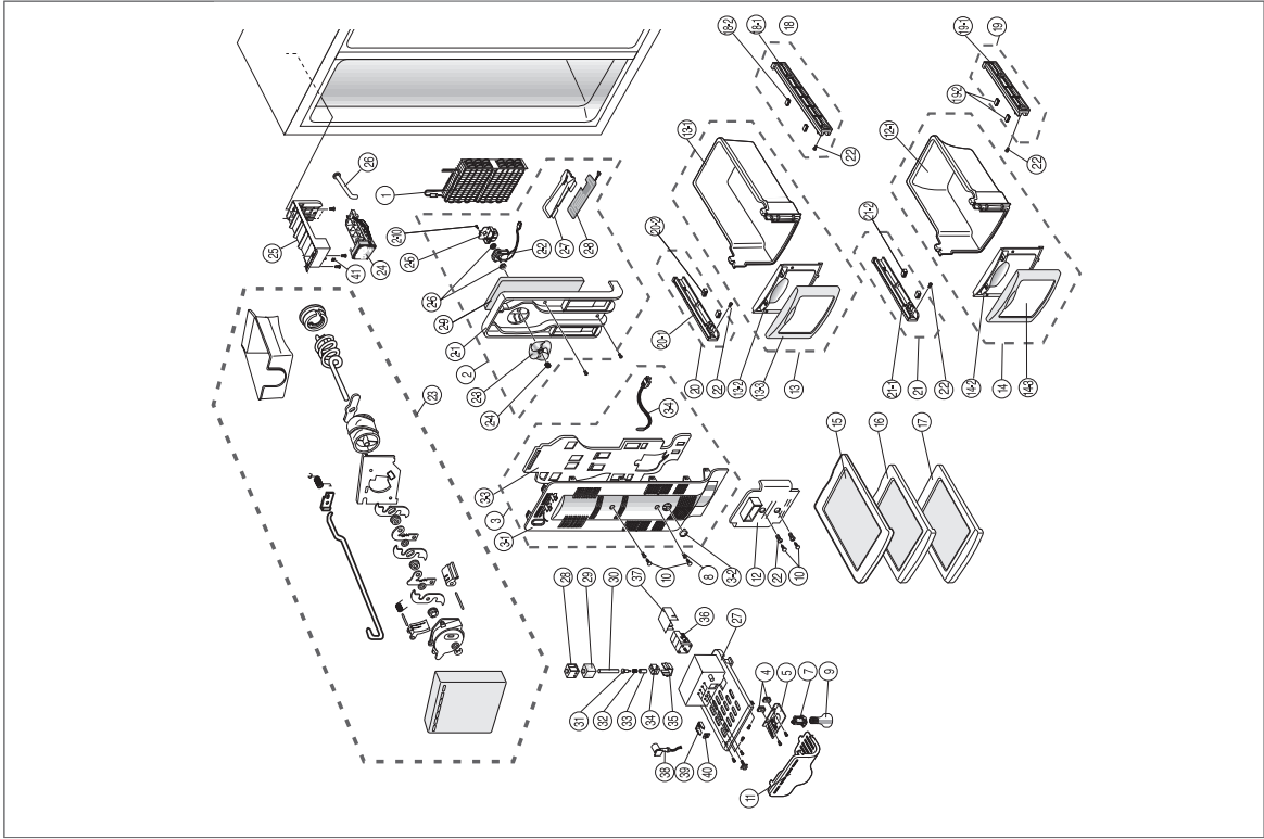
15-12 Freezing Compartment (SR-S24/25FTA)
