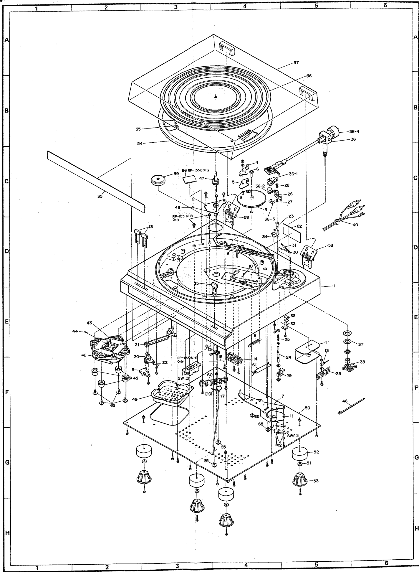
Figure 10 CABINET EXPLODED VIEW
