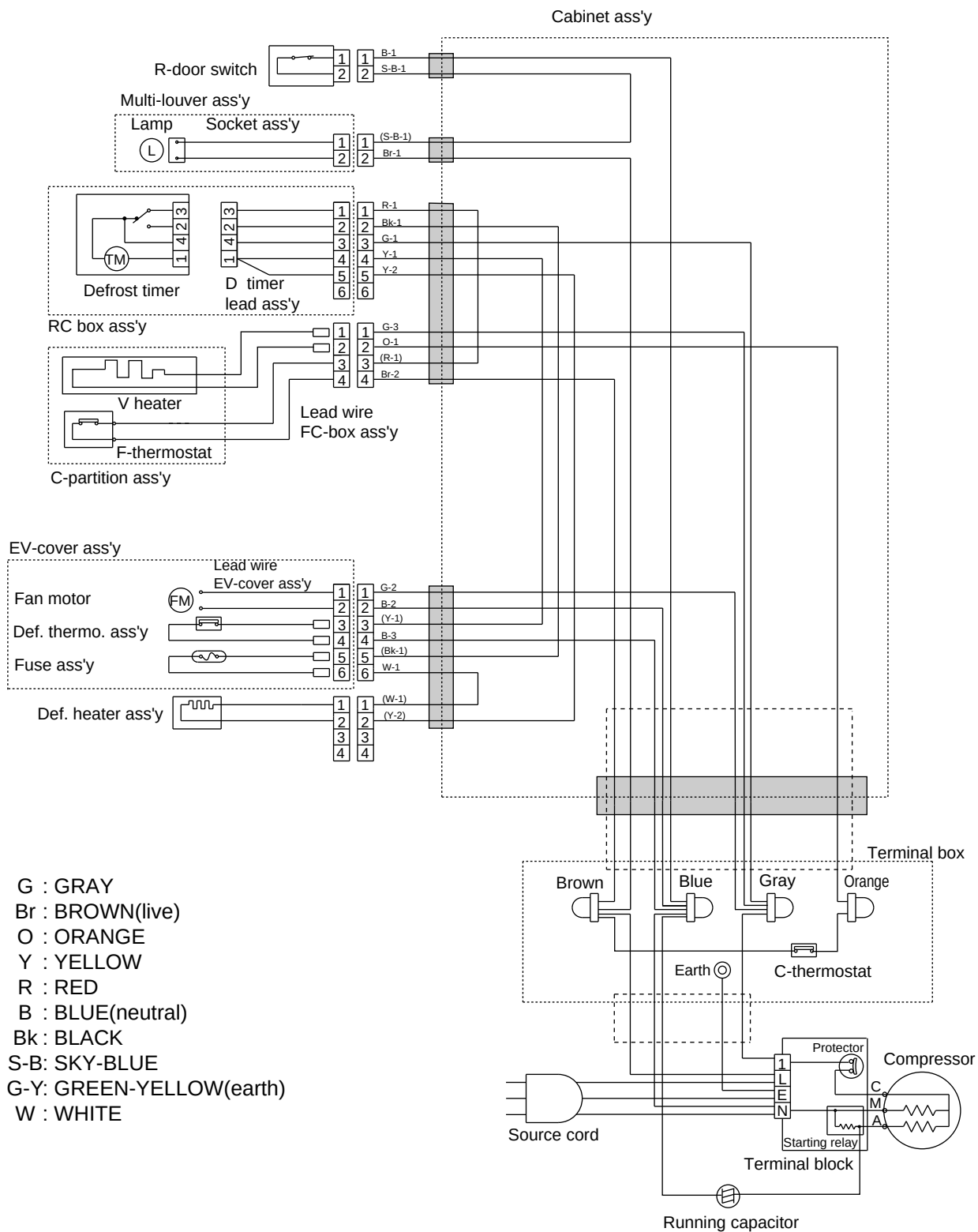
Figure W-2. Electric Accessories Layout
