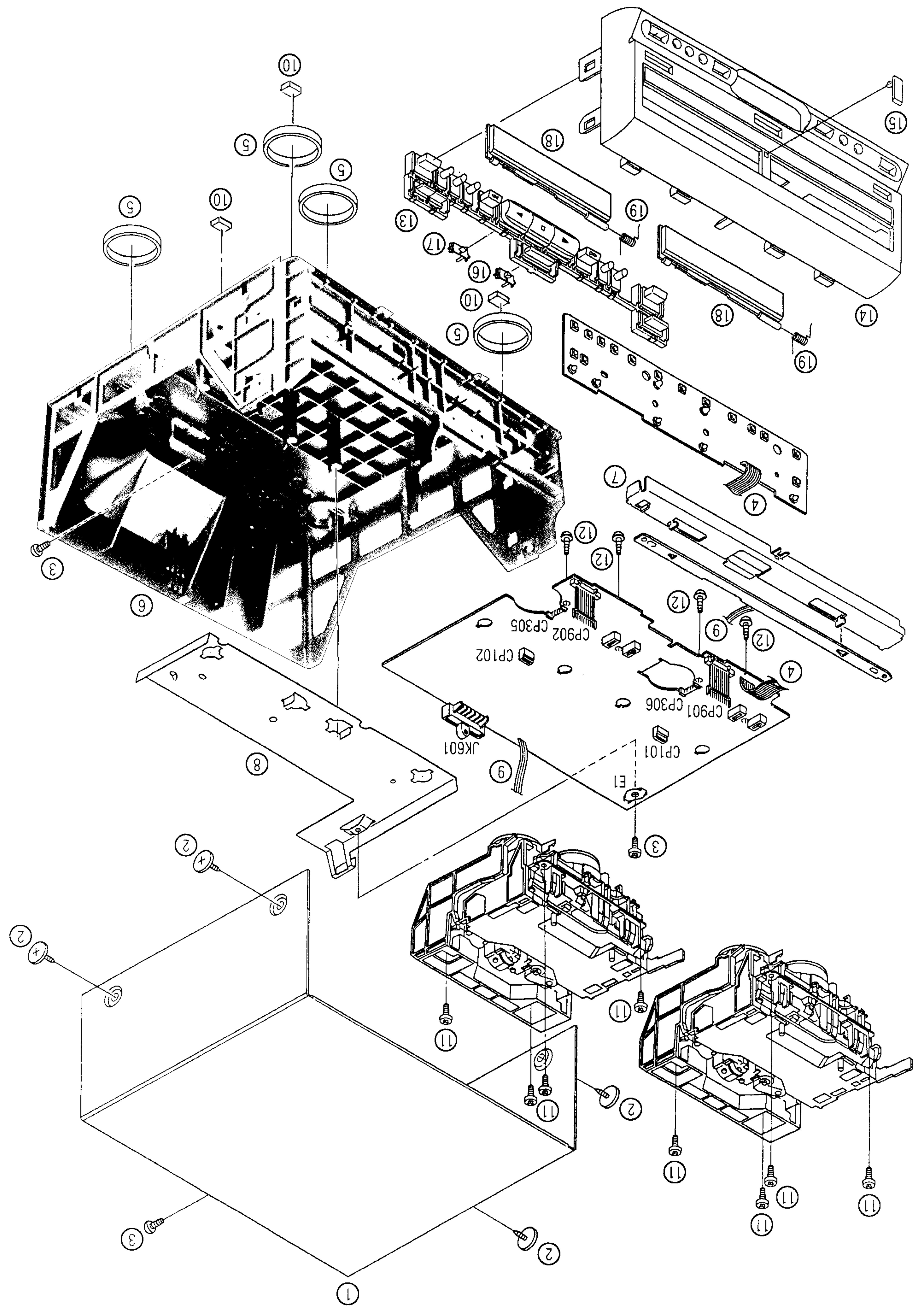
■ Cabinet Parts Location
