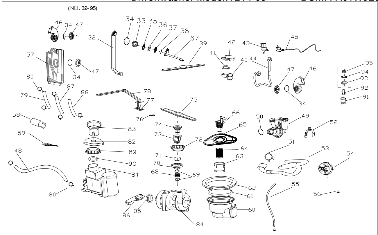
Exploded View
