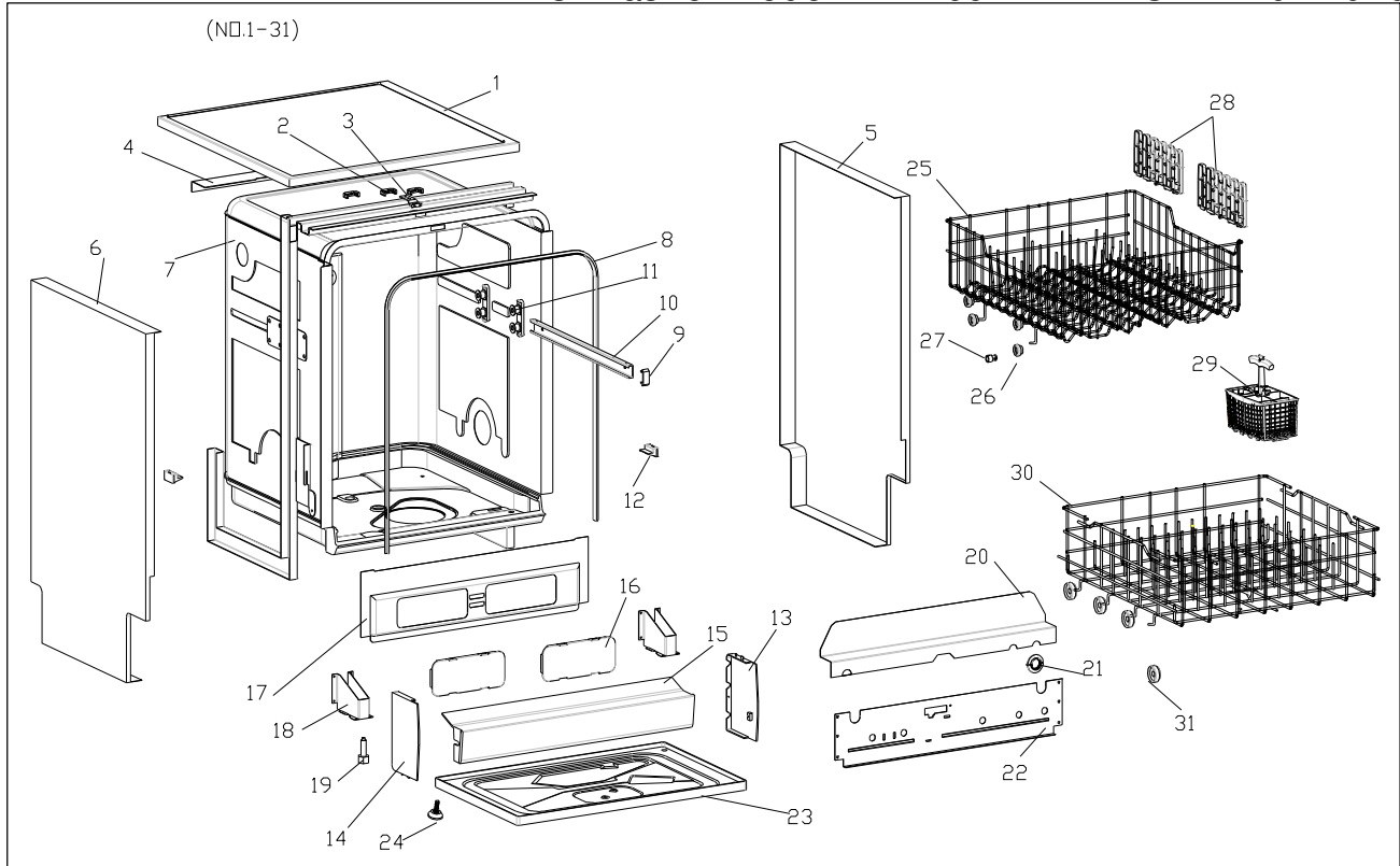
Exploded View
