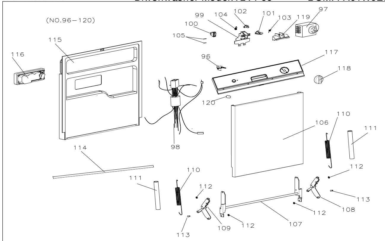
Exploded View
